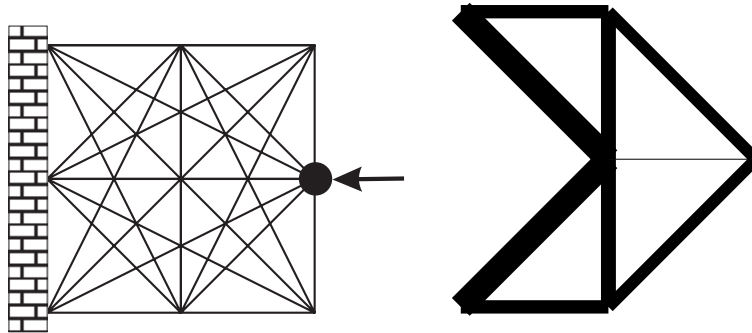
Figure 3: Three-by-three truss with nonstructural mass (Ex. 4.2): initial layout and optimal topology
