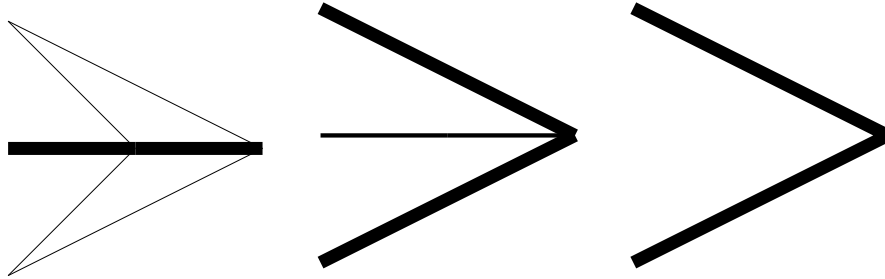
Figure 9: Example 4.6 demonstrating the dependence of the optimal structure on nonstructural mass changes; optimal results for M_0 = 0, 10, 100 are depicted left-to-right.
