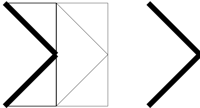
Figure 8: Example 4.5—optimal structures for x_i \geq 2 \cdot 10^{-3} (left) and x_i \geq 0 (right).
