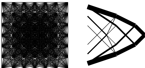
Figure 11: Example 4.8—a medium-size problem, initial layout and optimal topology
