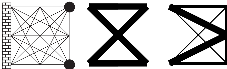
Figure 13: A multiple-mass problem (Ex. 5.1: initial layout (left), a “single-mass” result (middle) and a multiple-mass optimal structure (right)
