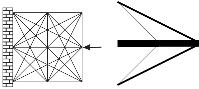
Figure 2: Three-by-three truss (Ex. 4.1): initial layout and optimal topology
