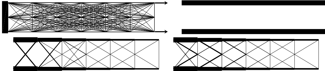
Figure 10: A medium size multiple-load example (Ex. 4.7): initial layout (top-left); optimal topology without (top-right) and with (bottom-left) vibration constraints; single-load optimal result with vibration constraints (bottom-right)
