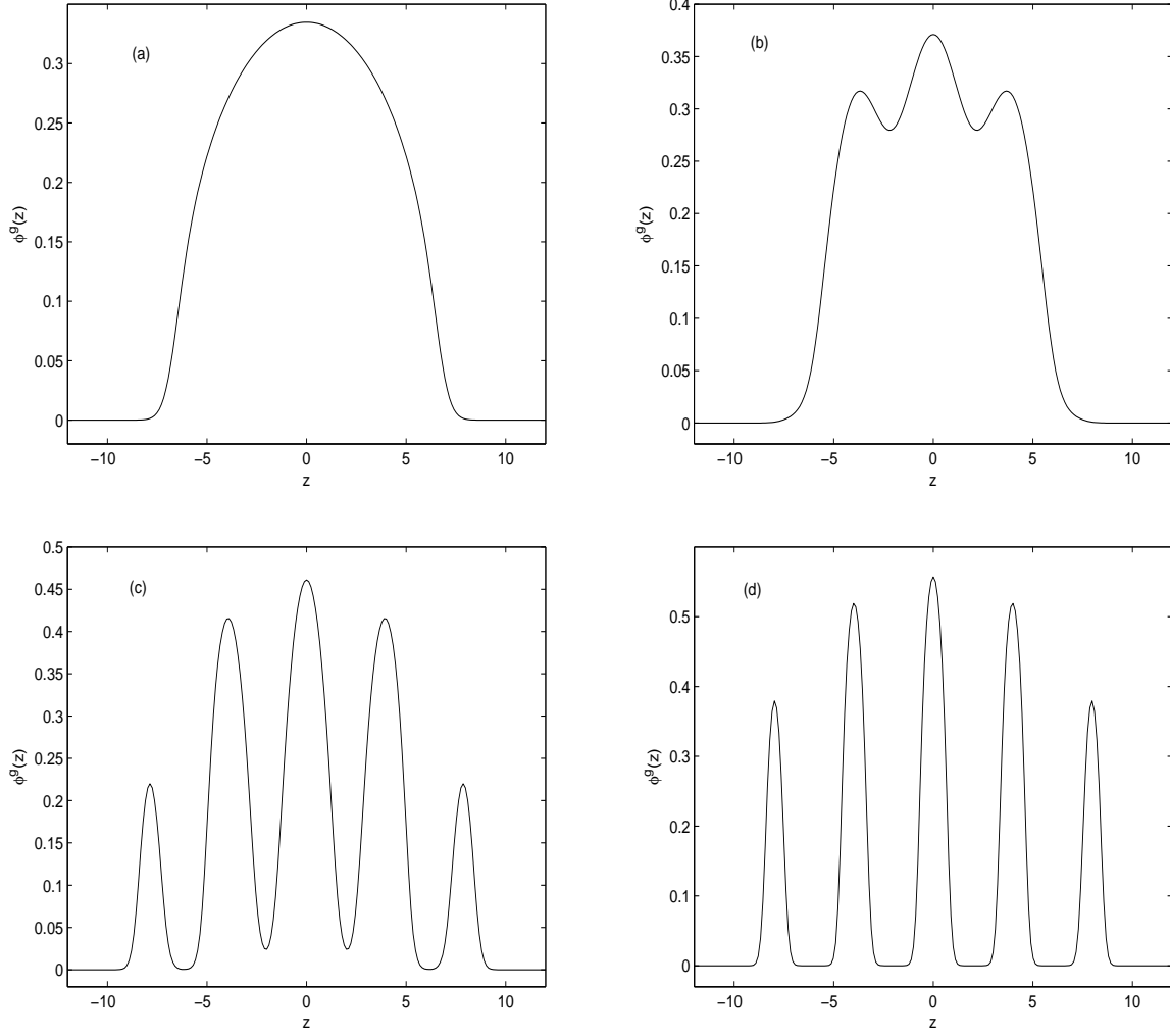
FIGURE 4. Ground states of 1D BEC with \beta_1 = 200 and W(z) = V_0 \sin^2(\pi z/4) for different V_0 : (a) V_0 = 0 ; (b) V_0 = 10 ; (c) V_0 = 50 ; and (d) V_0 = 200 .
