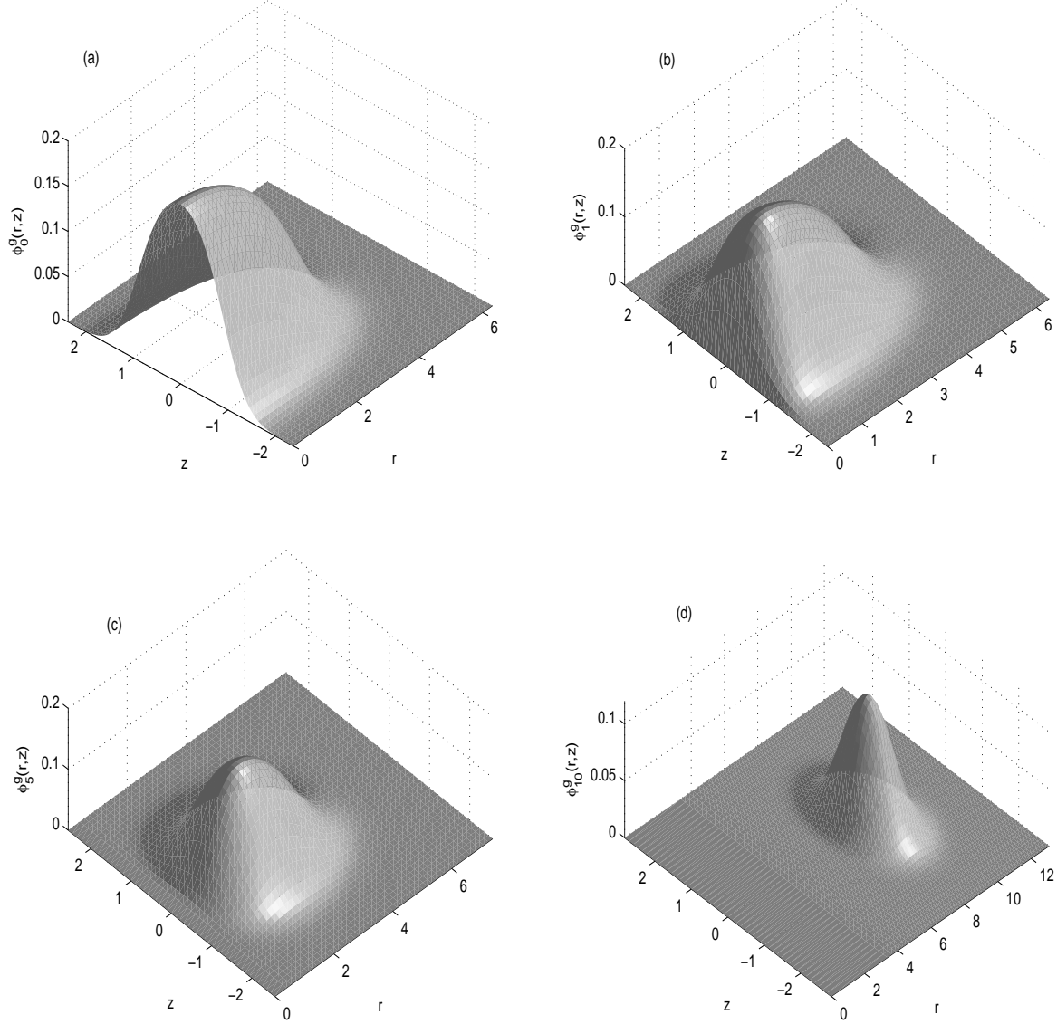
FIGURE 5. Symmetric and central vortex line states of 3D BEC with cylindrical symmetry with \gamma_r = 1 , \gamma_z = 4 , W(z) \equiv 0 and \beta = 200 for different m : (a) m = 0 ; (b) m = 1 ; (c) m = 5 ; and (d) m = 10 .
