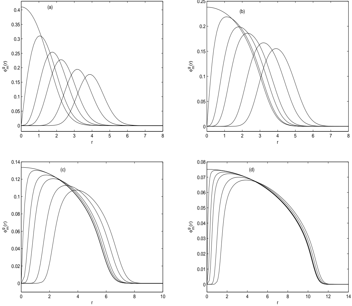
FIGURE 2. Symmetric and central vortex states of 2D BEC with radial symmetry for m = 0, 1, 3, 5, 10, 15 (in the order of decreasing of peak values) and different \beta_2 : (a) \beta_2 = 10 ; (b) \beta_2 = 100 ; (c) \beta_2 = 1000 ; and (d) \beta_2 = 10000 .
