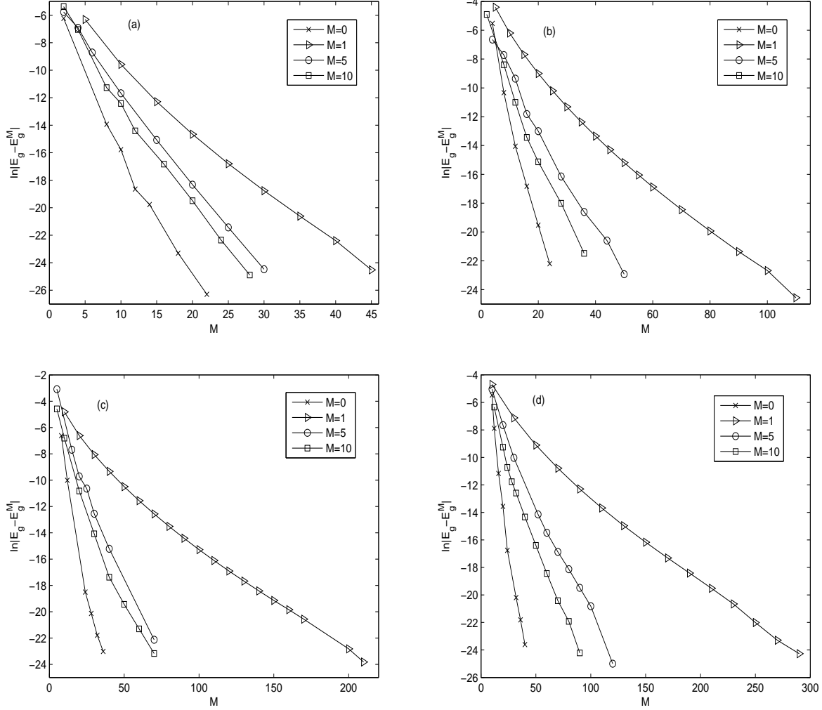
FIGURE 1. Error analysis for computing symmetric and central vortex states of 2D BEC with radial symmetry by using (4.25) for different m and \beta_2 : (a) \beta_2 = 10 ; (b) \beta_2 = 100 ; (c) \beta_2 = 500 ; and (d) \beta_2 = 1000 .
