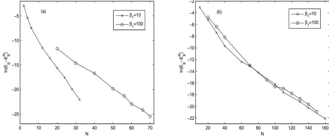
FIGURE 3. Error analysis for computing ground states of 1D BEC with W(z) = V_0 \sin^2(\pi z/4) by using (4.10) for different \beta_1 and V_0 : (a) V_0 = 0 ; and (b) \beta_2 = 25 .
